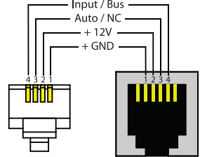
RJ11 (6p4c)
